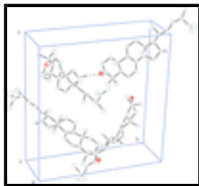
Fig. 2. Unit cell packing of (I) showing non-classical hydrogen bonding interaction with dashed lines; H atoms not involved in H-bonds have been excluded for clarity.
