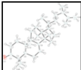
Fig. 1. ORTEP-3 (Farrugia, 1997) drawing of (I) with displacement ellipsoids plotted at 50% probability level.
